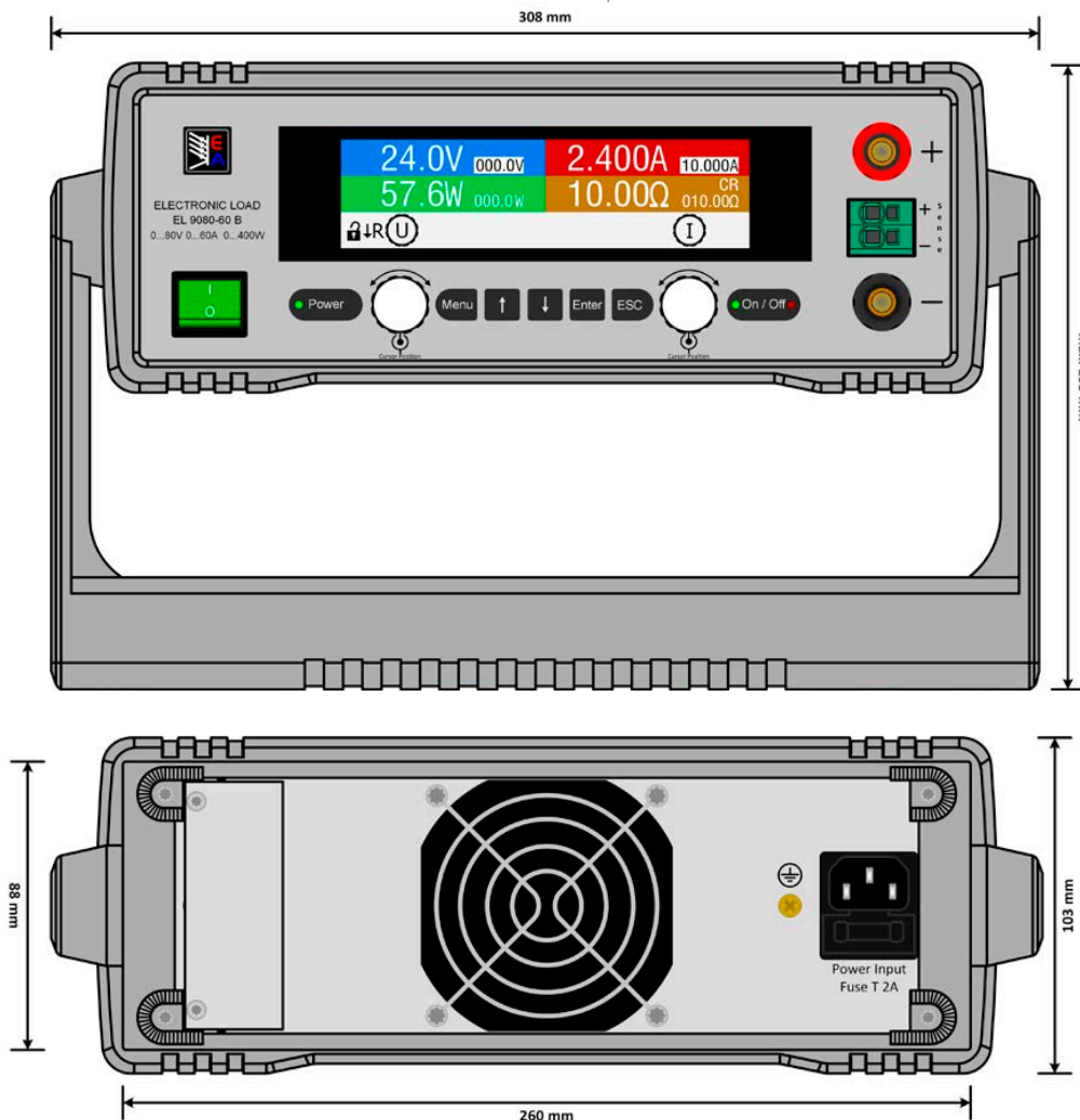
标配版的后视图 / Rear view of the standard configuration
